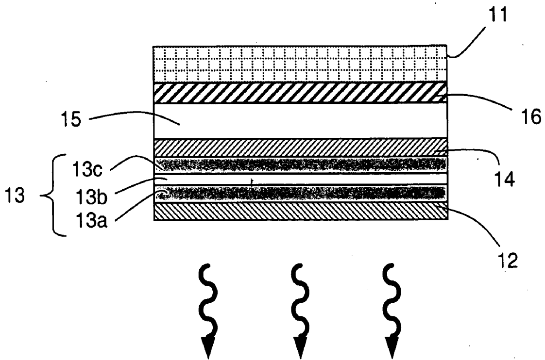
FIG. 1 – PRIOR ART
